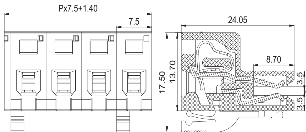
KF2EDGDJ-7.5
