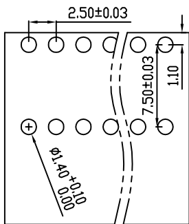
PCB LAYOUT
