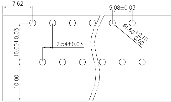
PCB LAYOUT
