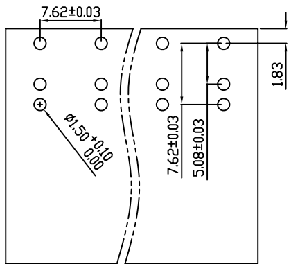
PCB LAYOUT
