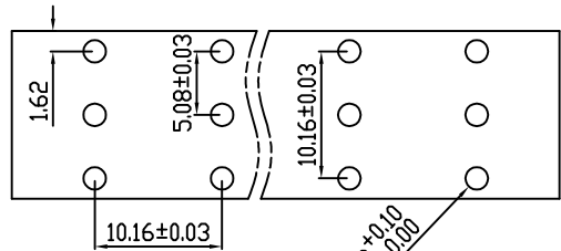
PCB Layout
