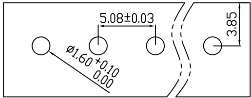
PCB LAYOUT
