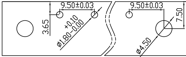
PCB LAYOUT
