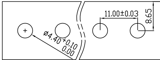
PCB LAYOUT
