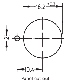
Panel cut-out
