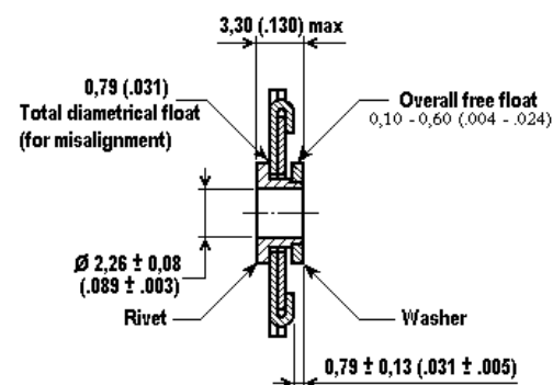
Dimension K – Receptacle
