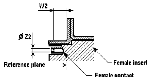
Female connector
