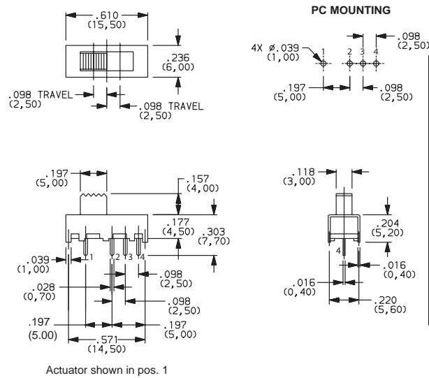
OS103012MU2QP1 SP3T
