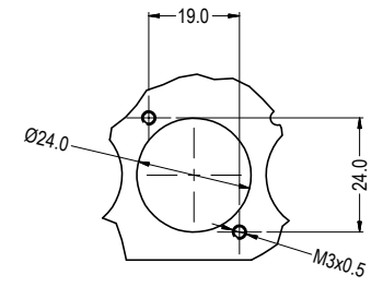
DETAIL VIEW A (32x POSITIONS)
