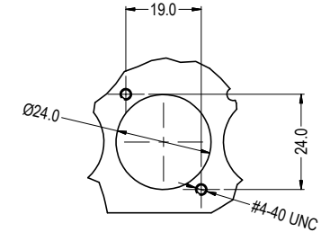
DETAIL VIEW A (32x POSITIONS)
