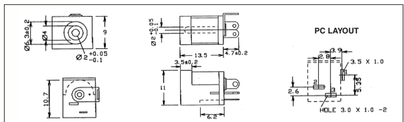
DC-9 PCB mounting pin ring type with switch. Rated 12V / 5A. DC9 with 2.1mm dia. pin. DC9A with 2.5mm dia. pin.
