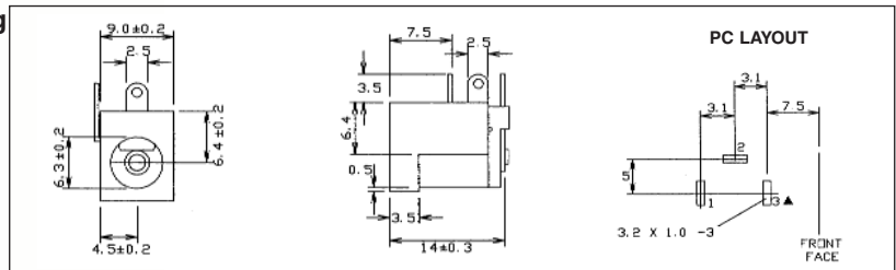
DC-10 PCB mounting pin / ring type with switch. Rated 12V / 5A. DC10A with 2.1mm dia. pin. DC10B with 2.5mm dia. pin.
