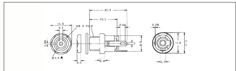
SCD-026 chassis mounting. SCD - 026 with 2.1mm dia. pin. SCD - 026A with 2.5mm dia. pin.
