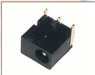
DC-8 PCB mounting pin ring type. Rated 12V / 1A. Miniature version for PCB mounting. 1.3mm dia. pin.
