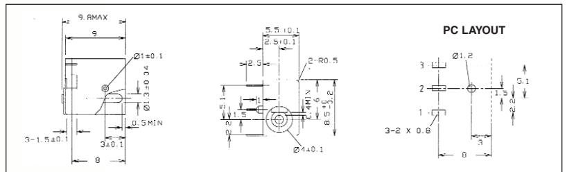
DC-8 PCB mounting pin ring type. Rated 12V / 1A. Miniature version for PCB mounting. 1.3mm dia. pin.
