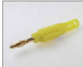
FCR7365Y P18 2mm PLUG UNSHROUDED YELLOW SUPPLIED UNASSEMBLED
