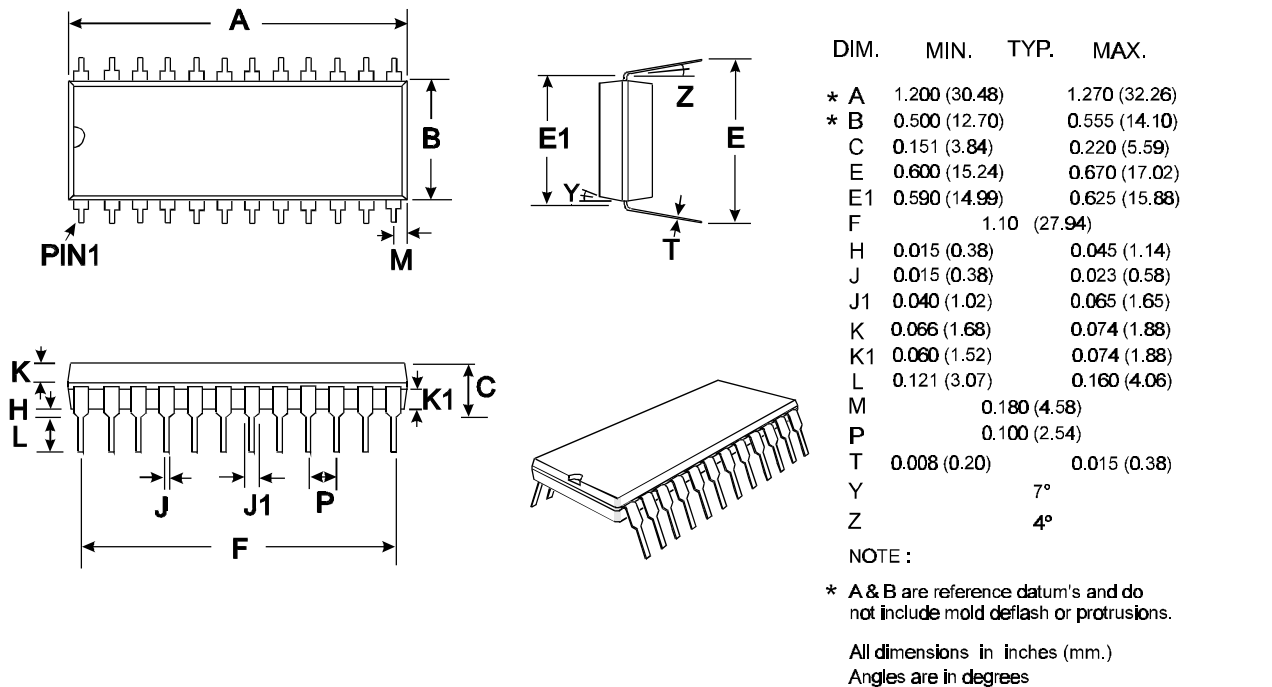
Figure 10 P4 Mechanical Outline: Order as part no. CMX641AP4
