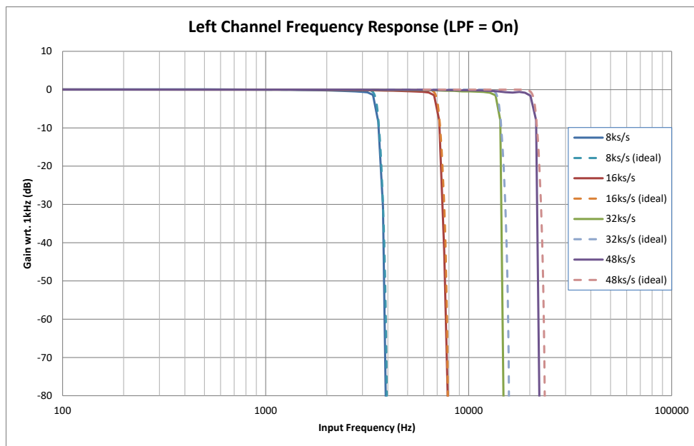
Figure 58 Low Pass Filter response Microphone Channels
