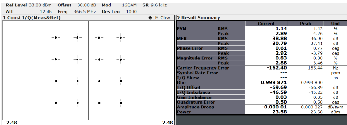
Figure 25 16-QAM, 9.6 ks/s, Constellation and EVM at 366.5MHz
