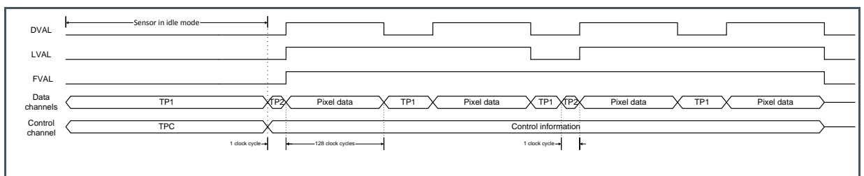
Figure 37 : TP Timing
