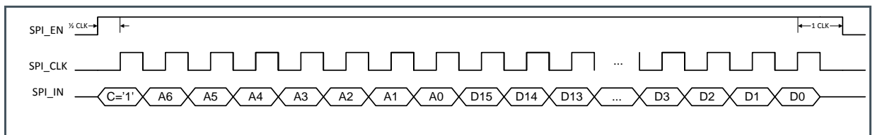
Figure 15 : SPI Write
