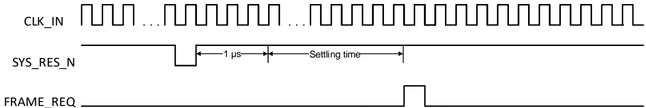
Figure 8: Reset sequence
