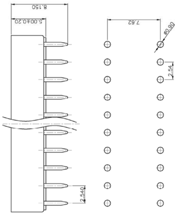
PCB LAYOUT
