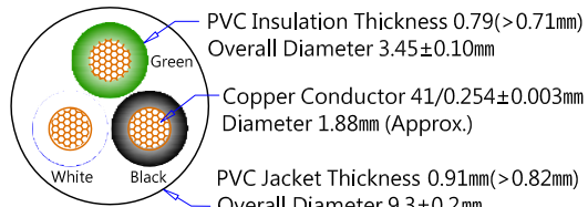
SJT 14AWGx3C 截面圖 (Wire Cross-Section)
