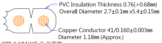
SPT-1 18AWGx2C截面圖 (Wire Cross-Section)
