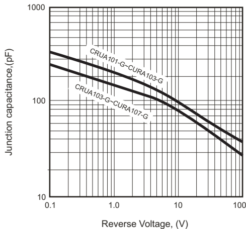
Fig.5 - Junction Capacitance
