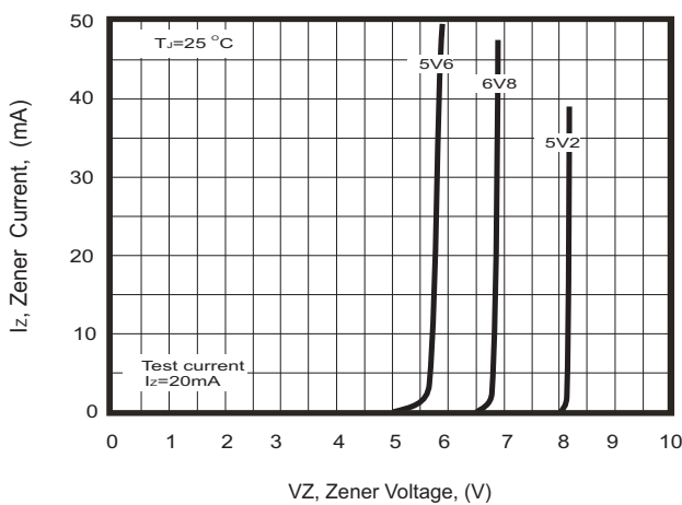
Fig.5- Zener Breakdown Characteristics
