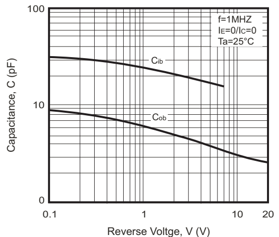
Fig.7 - C_{ob}/C_{ib} - V_{CB}/V_{EB}
