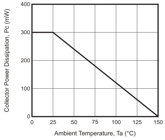
Fig.8 - P_c — T_a
