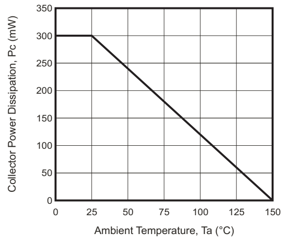
Fig.8 - P_c — T_a
