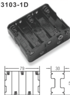
BH3103-1A BH3103-1B BH3103-1D FORTEN "AA" CELLS
