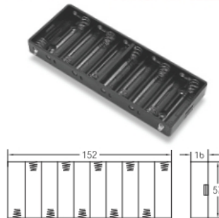
BH3101A BH3101D FORTEN "AA" CELLS
