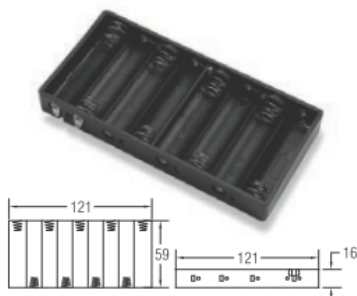
BH381A BH381B BH381D FOR EIGHT "AA" CELLS
