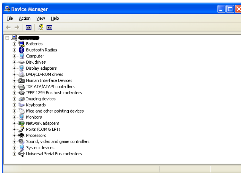
Figure 3-7 Device Manager
