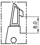
Standard latch
