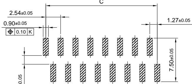
Recommended PC-Board layout (Component side of board shown)
