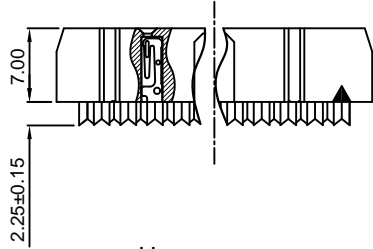
Upper cover
