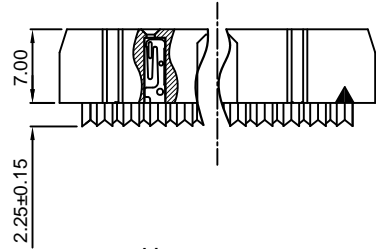
Upper cover
