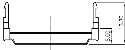
Top cover
