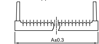
Upper cover
