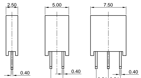
Single row N=No. of contacts Double row N=No. of contacts/2 Triplex row N=No. of contacts/3
