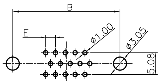
RECOMMEND PCB LAYOUT(TOLERANCE=±0.05) (VIEW FROM TOP SIDE)
