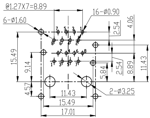
PCB LAYOUT THICKNESS=1.6mm
