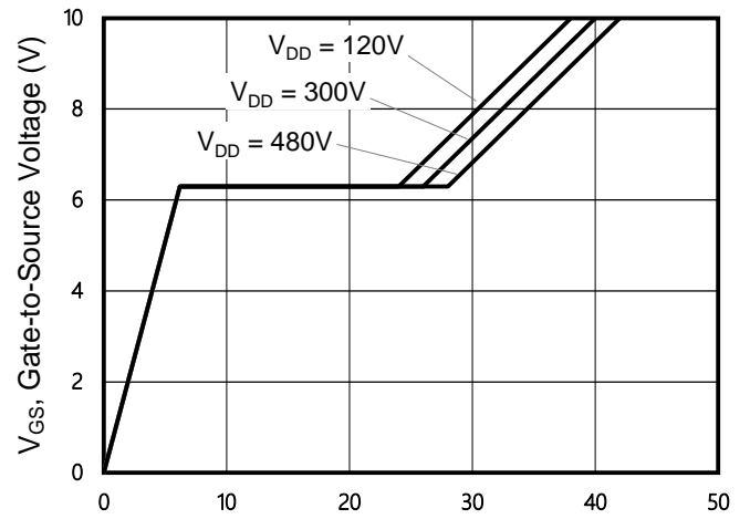
Figure 8. Gate Charge
