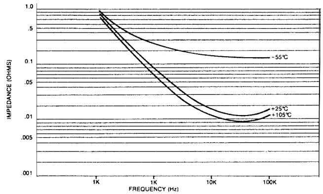
1500 µF 75V, 1" x 3 5 / 8 " Impedance-Frequency Characteristics
