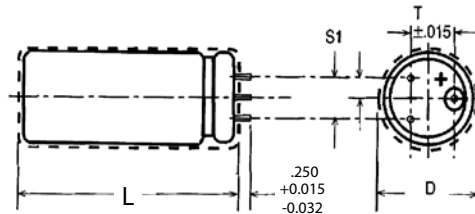
Type 300/300R Three Leads
