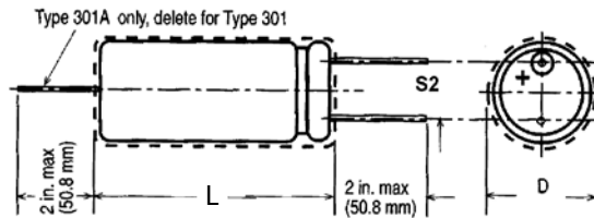
Type 301/301R Two Leads
