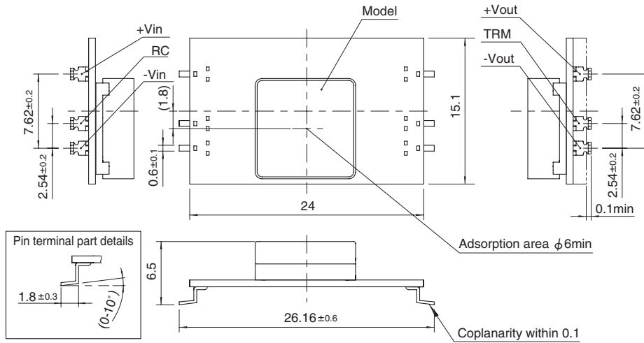
1. SMD (type B)
