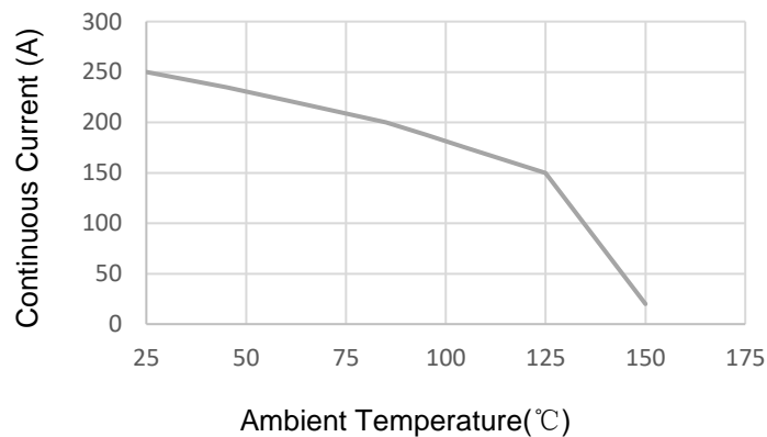
Figure 7: Maximum Continuous Current at a Given T_A
