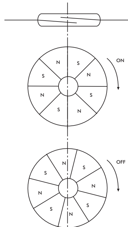
13.4: Rotational movement with two or more pole ring magnets
