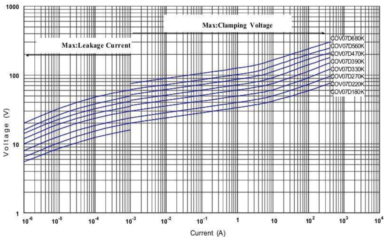
V-I Curve (COV07D180K to COV07D680K)
