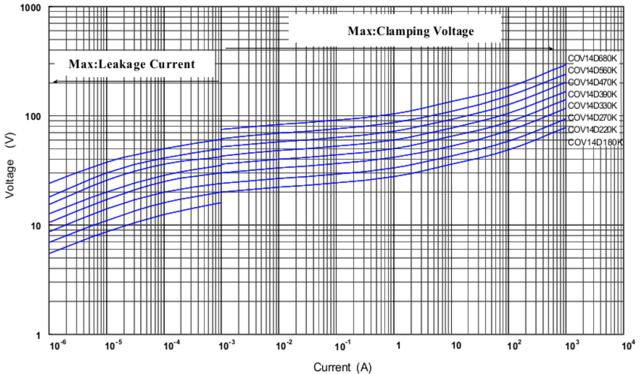
V-I Curve (COV14D180K to COV14D680K)
