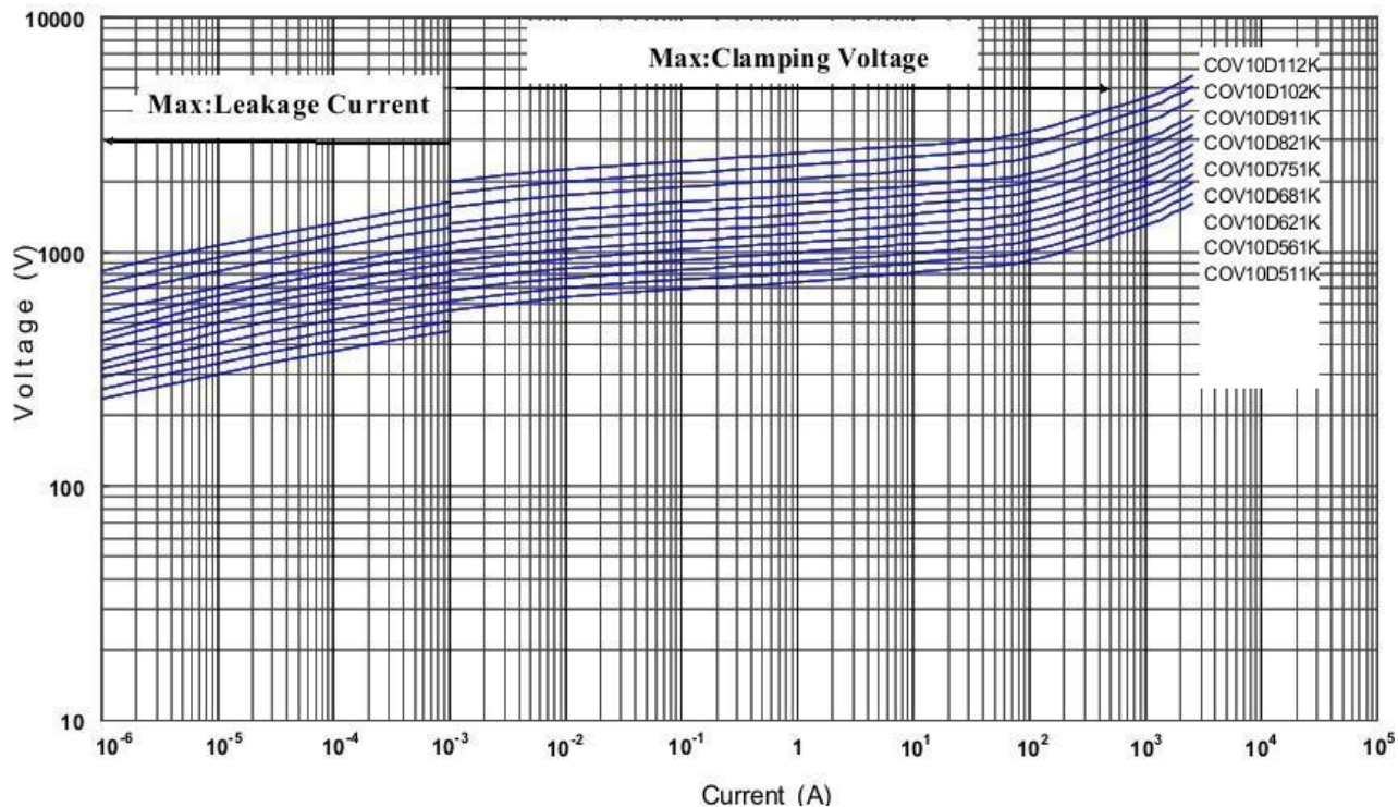
V-I Curve (COV10D511K to COV10D112K)
