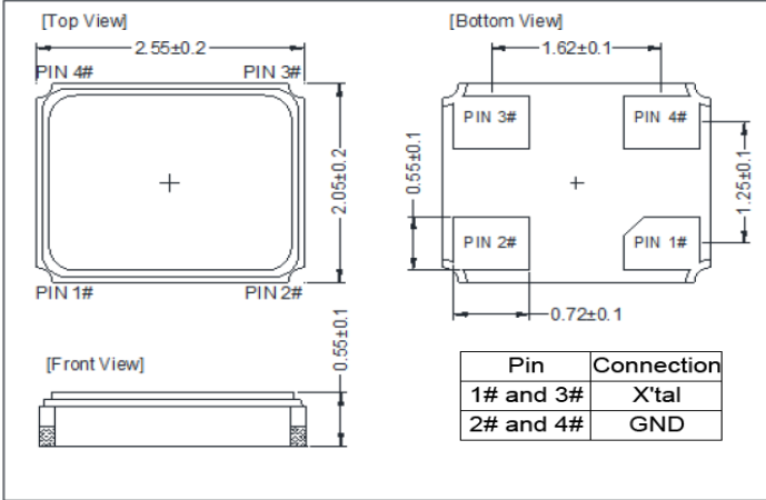
Product Dimensions
