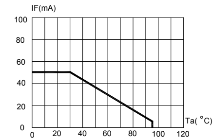
FIG.4 MAXIMUM FORWARD DC CURRENT VS AMBIENT TEMPERATURE ( T_{jmax}=105\text{ }^{\circ}\text{C} )
