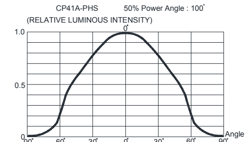
FIG.8 FAR FIELD PATTERN
