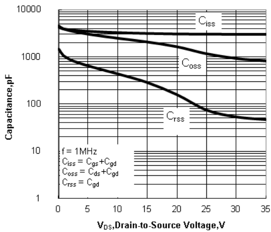
Figure 12. Capacitance Characteristics
